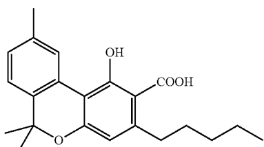
Cannabinolic acid (CBNA)
