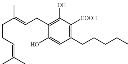
Cannabigerolic acid (CBGA)
