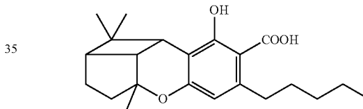
Cannabicyclolic acid (CBLA)
